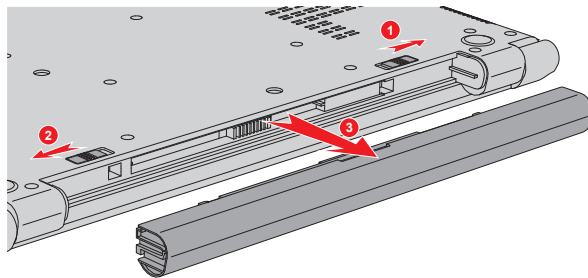
Figure 4-6 Releasing the battery pack
